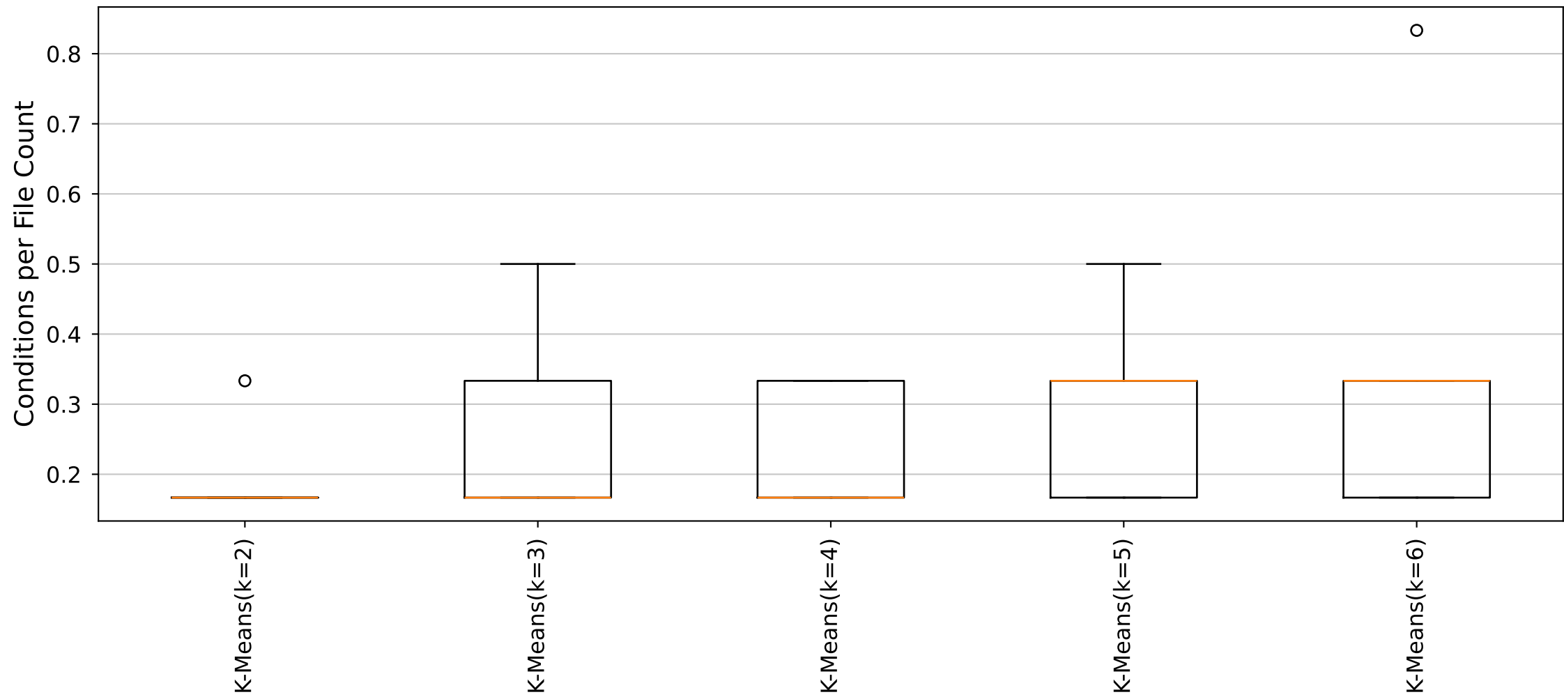
YARA Rules Conditions per File Count Distribution (Cluster21_Size6 dataset)
